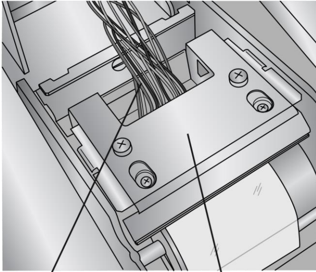
Disconnect this Cable Print Head Flipped 180 Degrees
